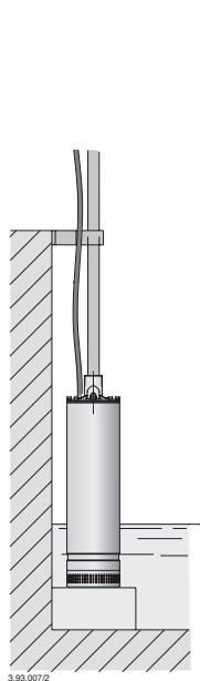
Fig. 1 Pompa appoggiata Pump in the standing position Pompe posée
