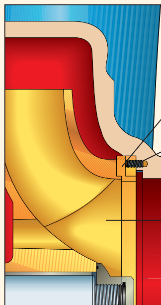
Enclosed Impeller Option
