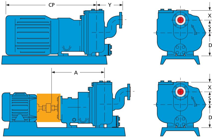
SP 3298 Frame-Mounted Design
