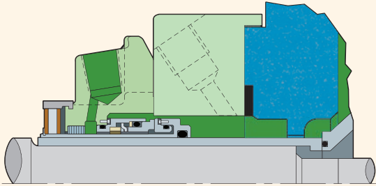
Single cartridge seal with backplate extension piece
