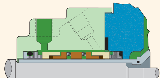
Double conventional seal with seal chamber extension
