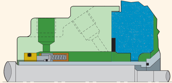
Single conventional seal with seal chamber extension
