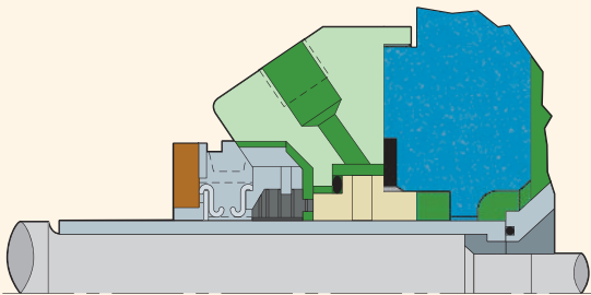
Single outside seal with clamped seat
