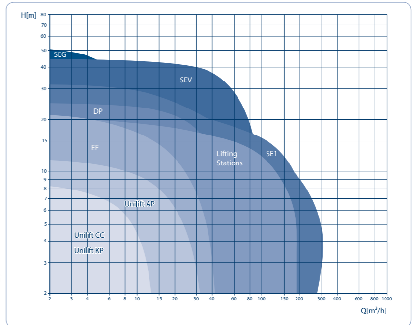
Pump performance
