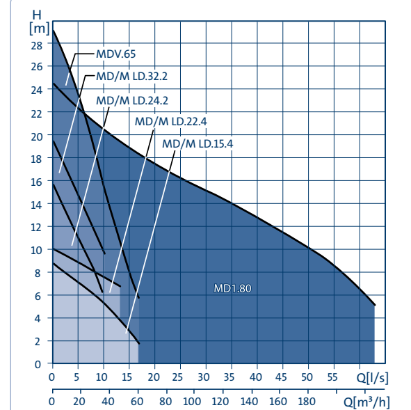
Pump performance
