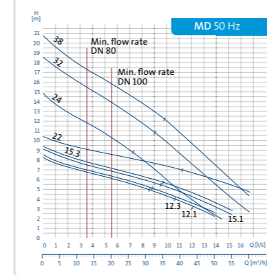
MULTILIFT MD
