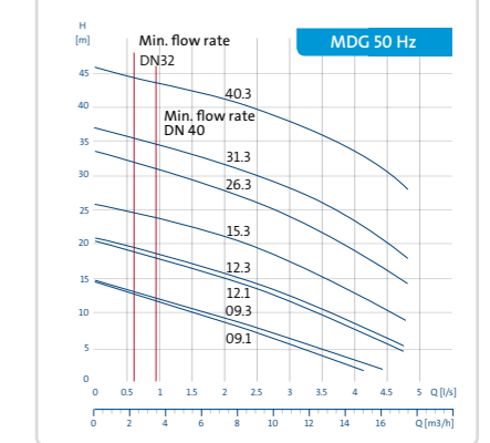
MULTILIFT MDG
