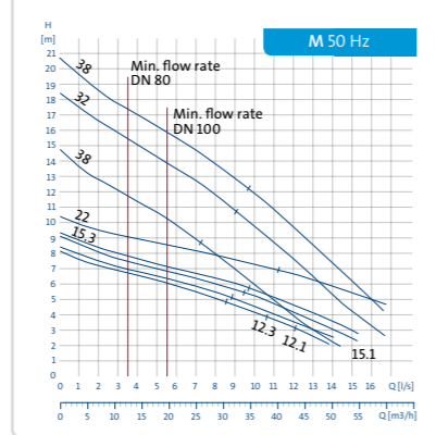
MULTILIFT M
