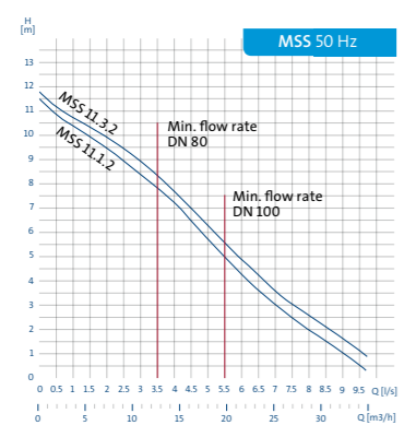
MULTILIFT MSS
