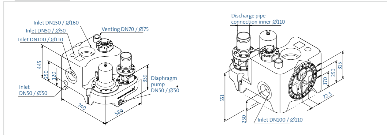
MULTILIFT M
