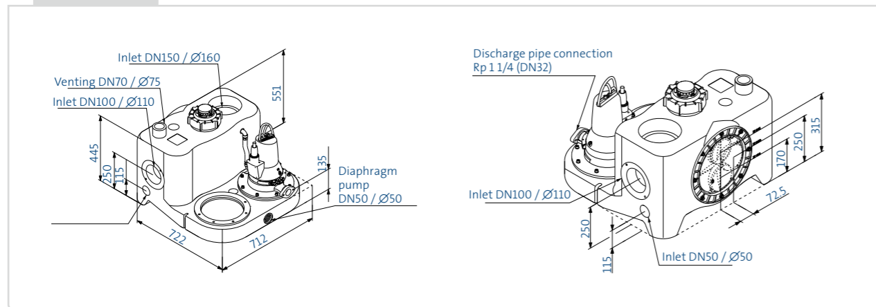
MULTILIFT MOG
