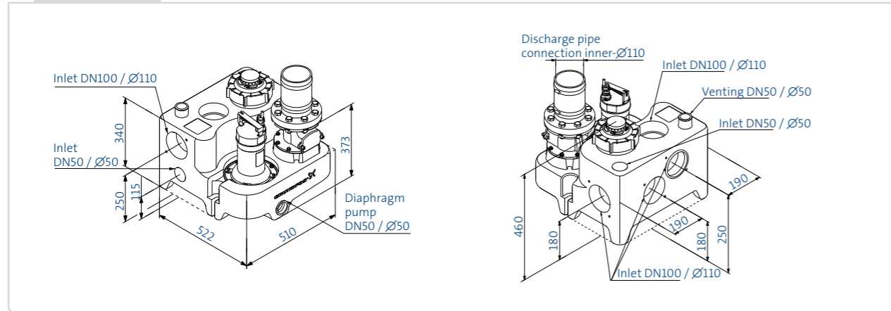
MULTILIFT MSS
