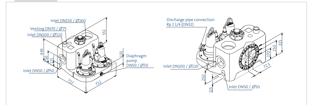
MULTILIFT MDG
