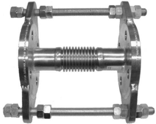
Fig. 22 Metal bellows expansion joint with limiting rods
