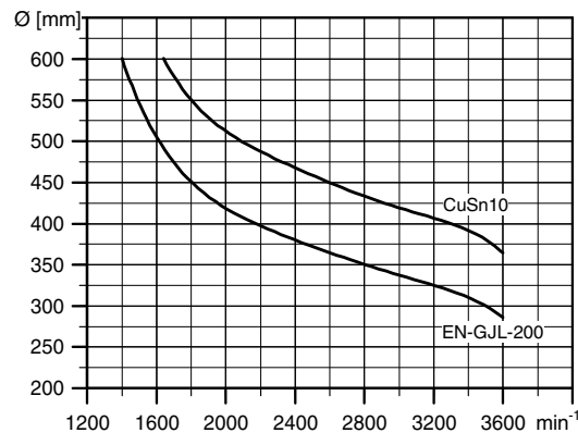
Fig. 7 Maximum permissible speed
