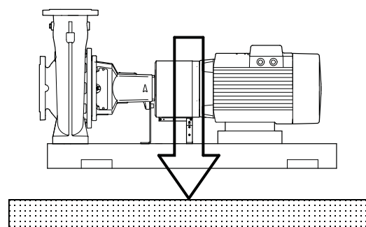
Fig. 13 Correct foundation
