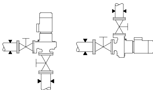
Fig. 18 Direct mounting in pipework
