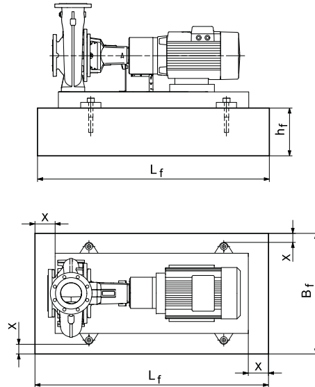
Fig. 12 Foundation, X = min. 100 mm
