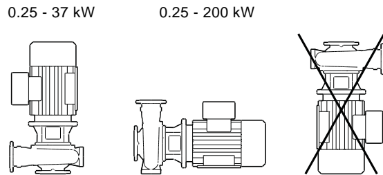
Fig. 10 Installation positions
