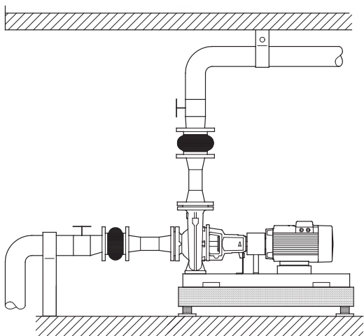
Fig. 17 Pipeline mounting
