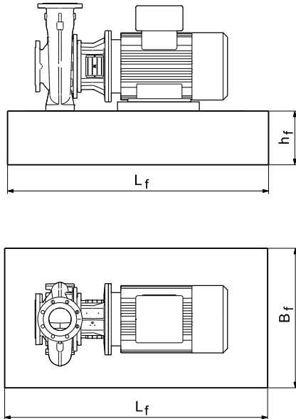
Fig. 11 Foundation
