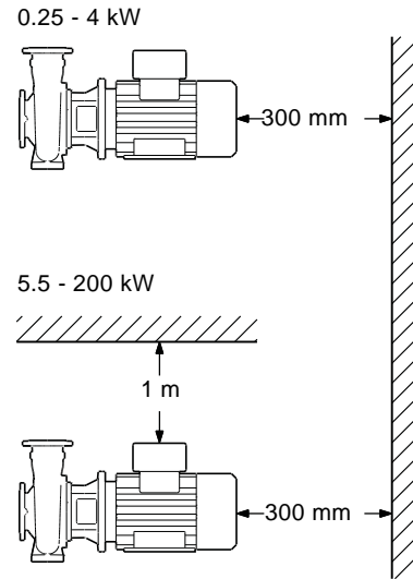
Fig. 9 Clearance behind the motor
