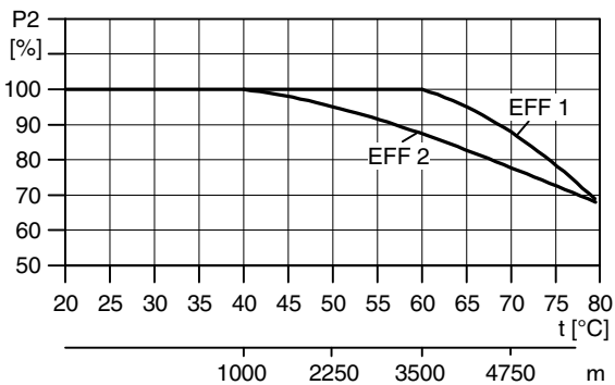
Fig. 6 Motor P2 in relation to temperature/altitude
