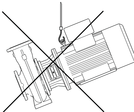
Fig. 3 Incorrect lifting of pump
