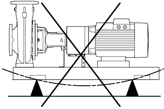
Fig. 14 Incorrect foundation
