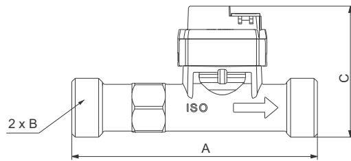
Fig. 67 Dimensions, VFS QT, 2-40 l/min, with threads
