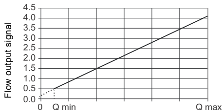
Fig. 64 Flow response in Analogue mode
