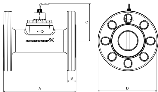
Fig. 27 Dimensions, VFI with flanges
