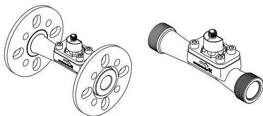
Fig. 7 VFI sensor with flanges and thread
