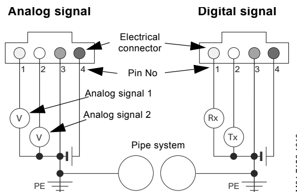
Fig. 33 Electrical connections
