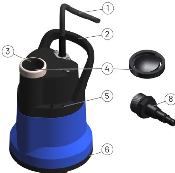
Simer 6 without level control
