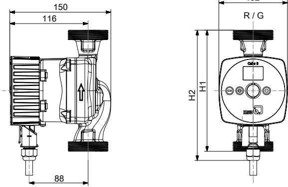
III. 4: Dimensions Calio S [mm]
