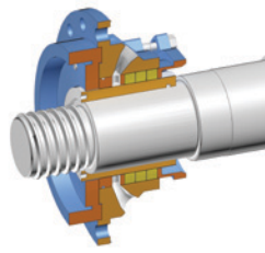
Throat Bushing
