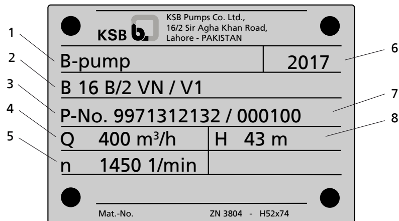
III. 1: Plaque signalétique (exemple)
