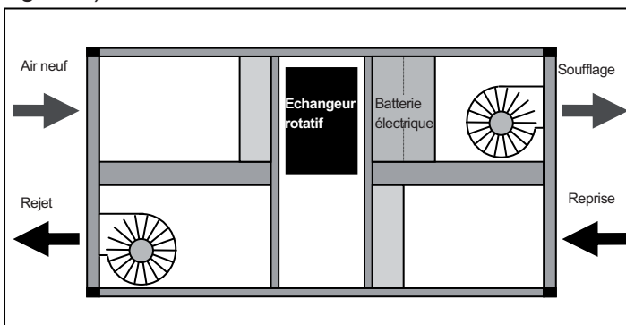
Figure 1 – Schema CAD O VL
