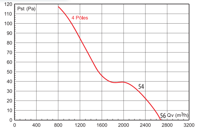
HCTB-HCTT 450 Extraction
