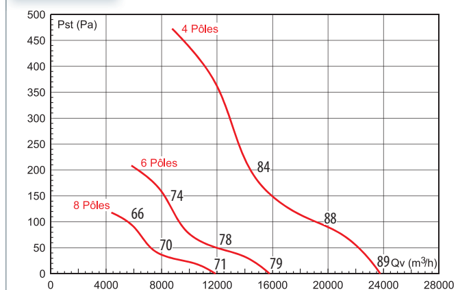
HCTT 800 Extraction
