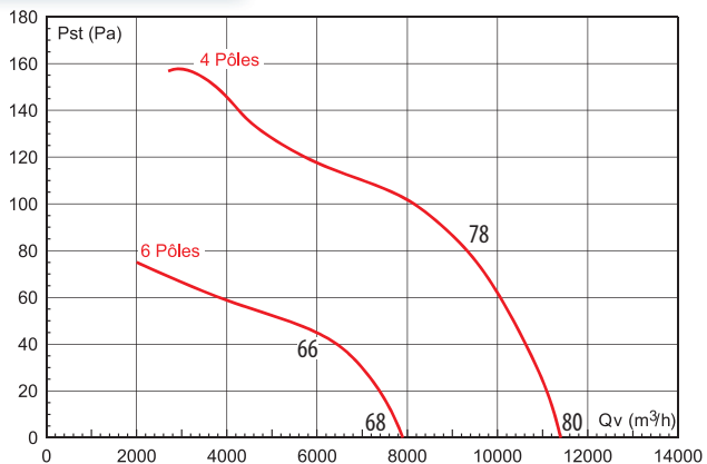
HCTB-HCTT 560 Insufflation
