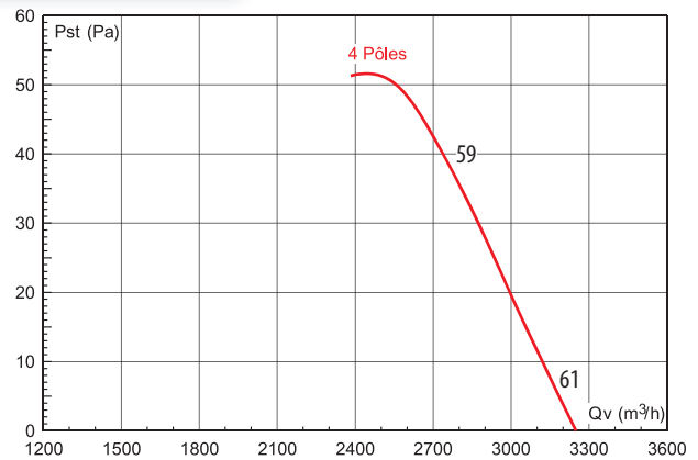
HCTB-HCTT 355 Insufflation
