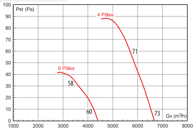
HCTB-HCTT 450 Insufflation
