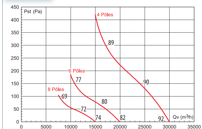
HCTT 900 Extraction
