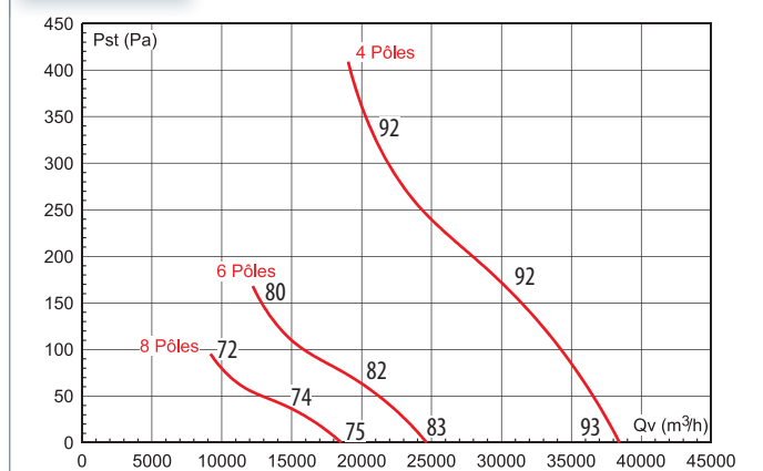
HCTT 1000 Extraction
