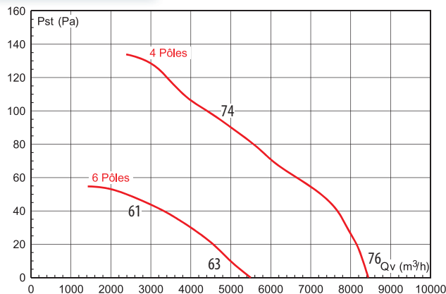
HCTB-HCTT 500 Insufflation
