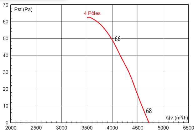
HCTB-HCTT 400 Insufflation
