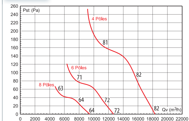
HCTT 710 Extraction
