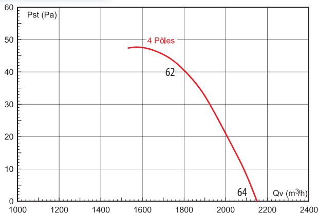
HCTB-HCTT 315 Insufflation
