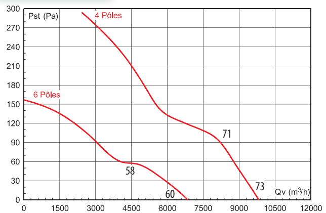
HCTB-HCTT 560 Extraction
