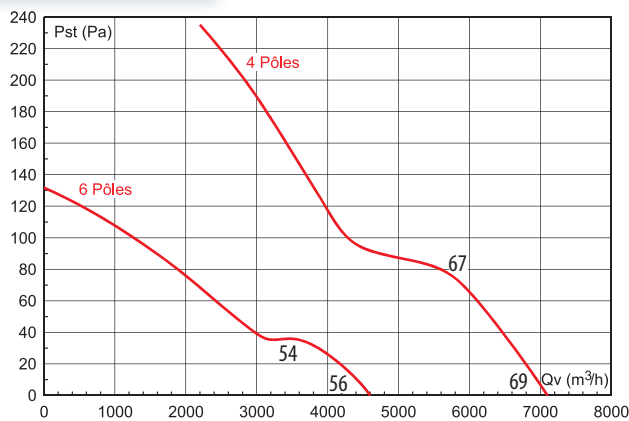
HCTB-HCTT 500 Extraction
