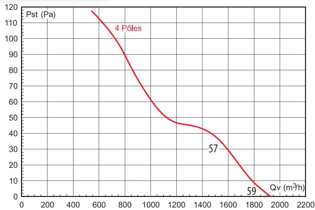
HCTB-HCTT 400 Extraction
