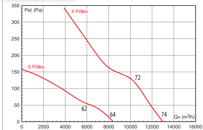
HCTB-HCTT 630 Extraction
