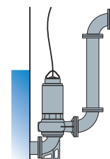
Dry with cooling system
